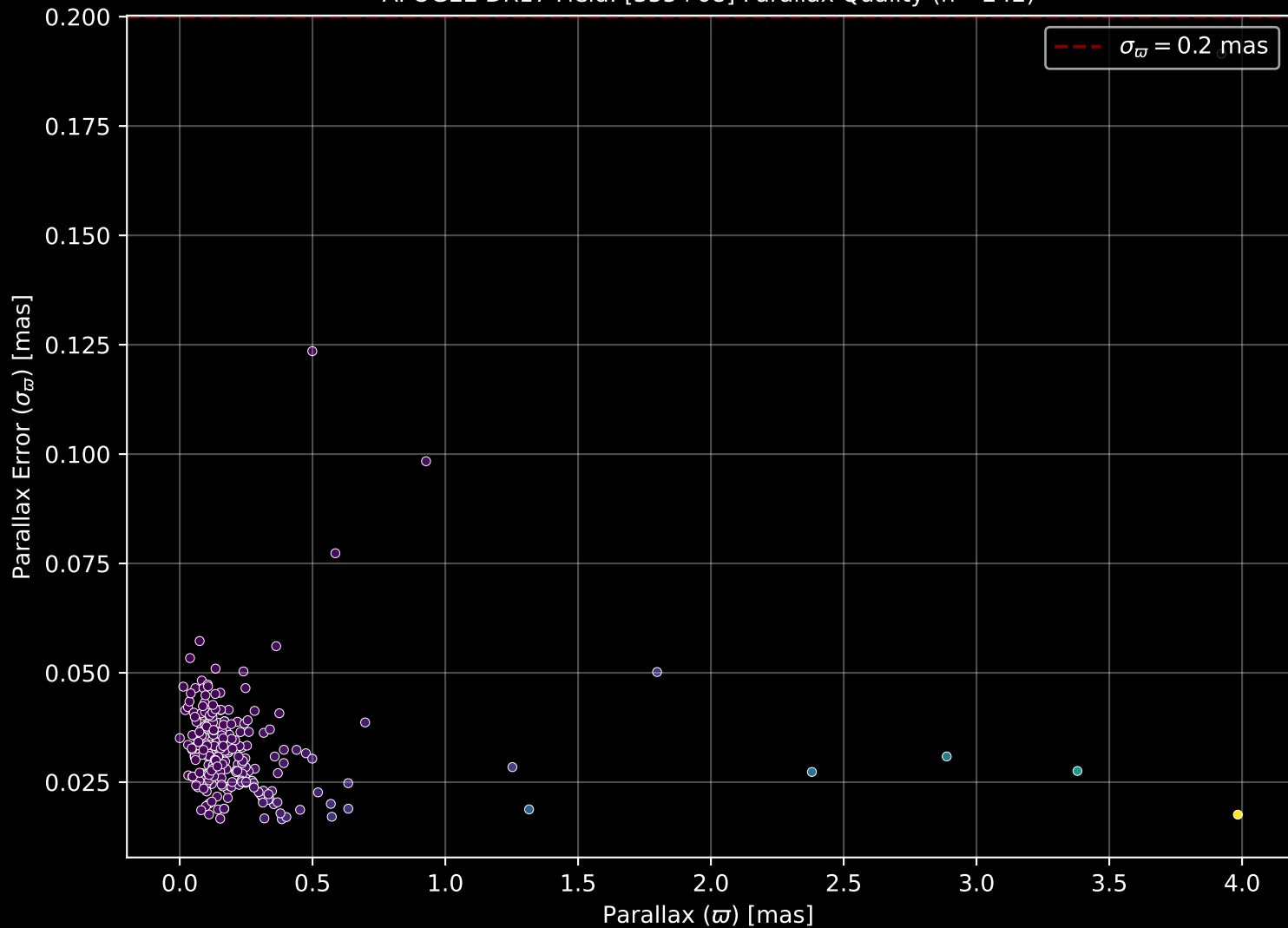
APOGEE DR17 Field: [355+08] Parallax Quality (n= 242)
