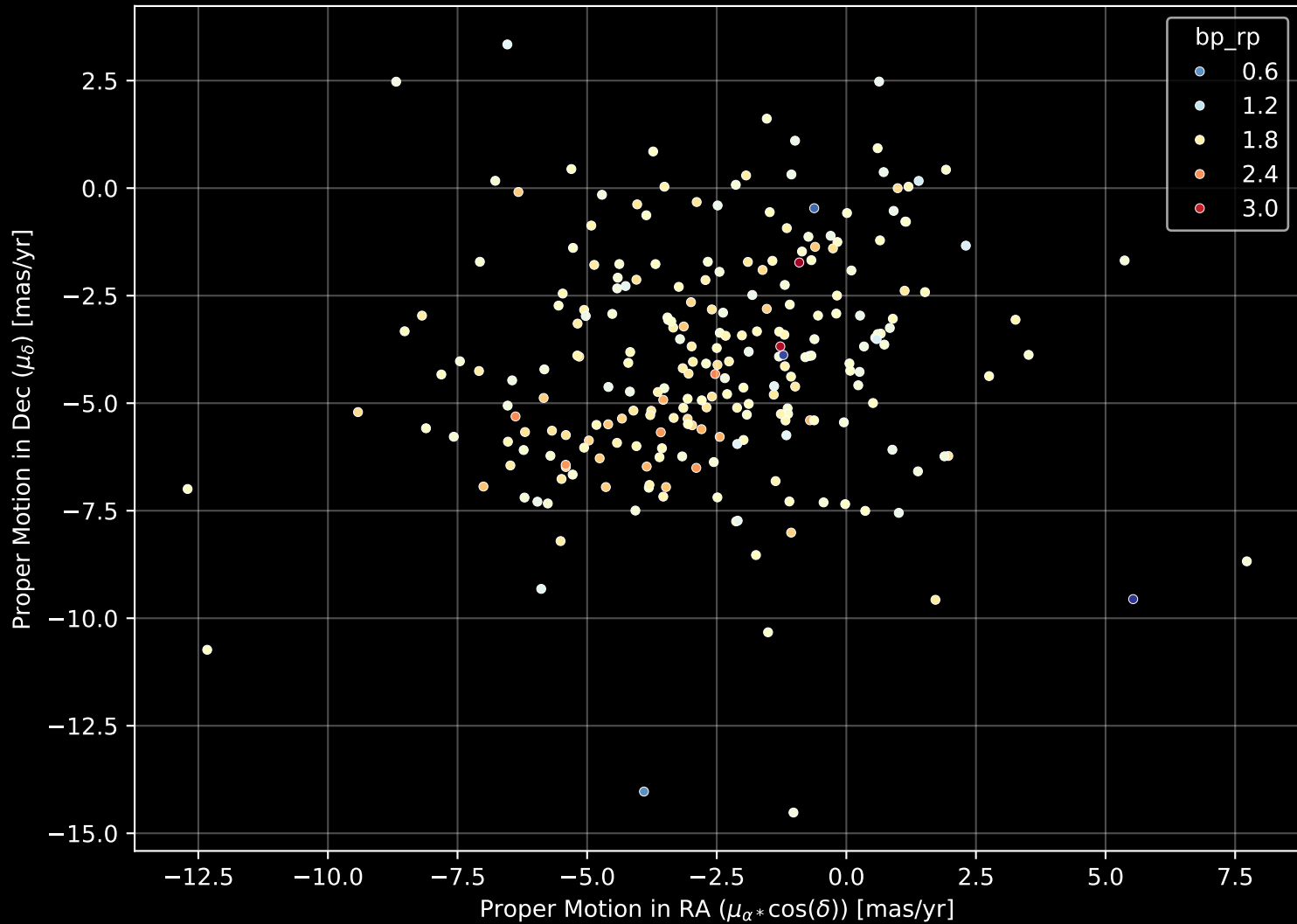
APOGEE DR17 Field: [355+08] Proper Motion Diagram (n= 242)
