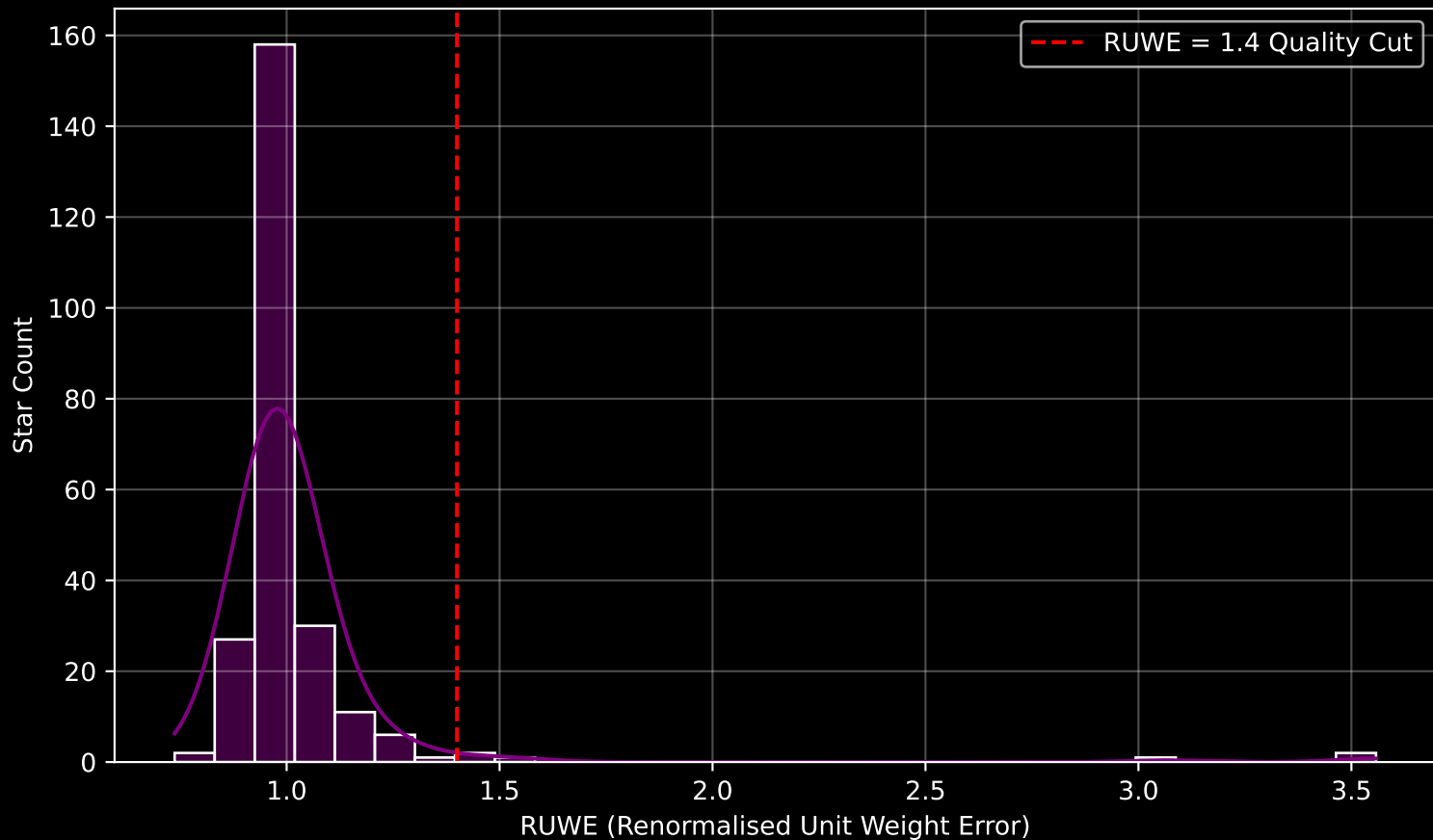
GAPOGEE DR17 Field [355+08] RUWE Distribution (n= 241)
