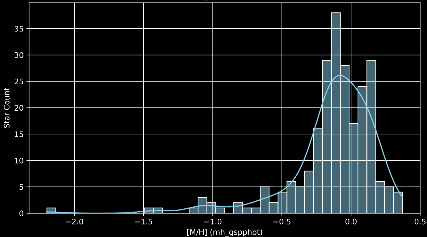
APOGEE DR17 Field: [355+08 [M/H] (mh_gspphot) (n= 240)
