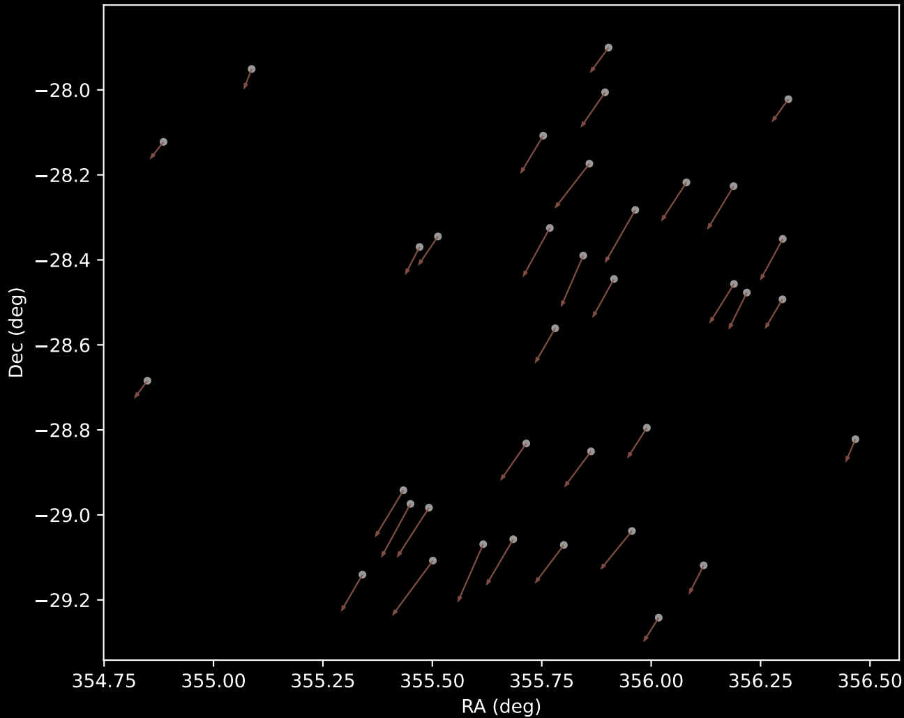
APOGEE DR17 Cluster 10 Proper Motion Vectors (n=36)
